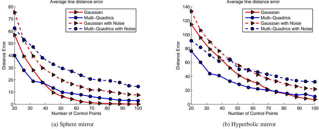
Figure 2: Evaluation of the average line distance error, Equation (24), as a function of the number of control points , for non-central catadioptric systems with sphere (a) and hyperbolic mirror (b). Dashed lines correspond to the average errors in the cases where Gaussian random noise was added to the coordinates.
